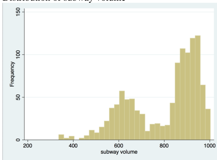
Figure 1: Distribution of subway volume
